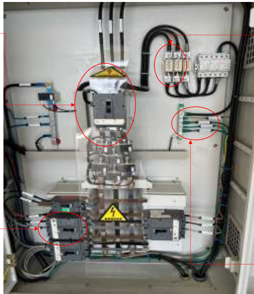
PV AC DB No.4 20SNPB-WAC01
